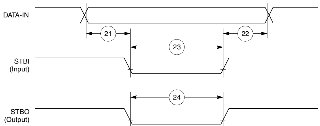
Figure 41. PIP Rx (Pulse Mode) Timing Diagram
