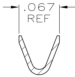
WIRE SIZE #22-#26 SECTION E-E
