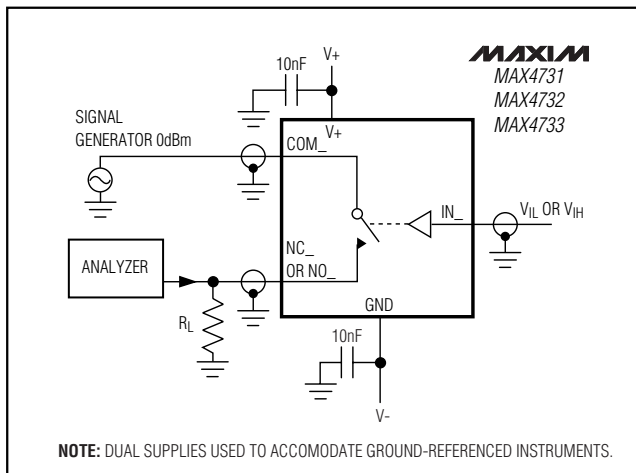
Figure 5. Off-Isolation/On-Channel Bandwidth
