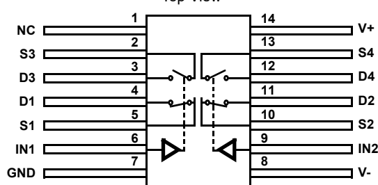
HS-303ARH, HS-303AEH, HS-303BRH, HS-303BEH (FLATPACK) CDFP3-F14 Top View
