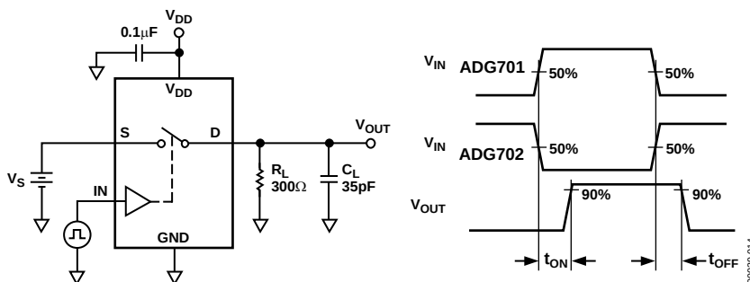
Figure 14. Switching Times
