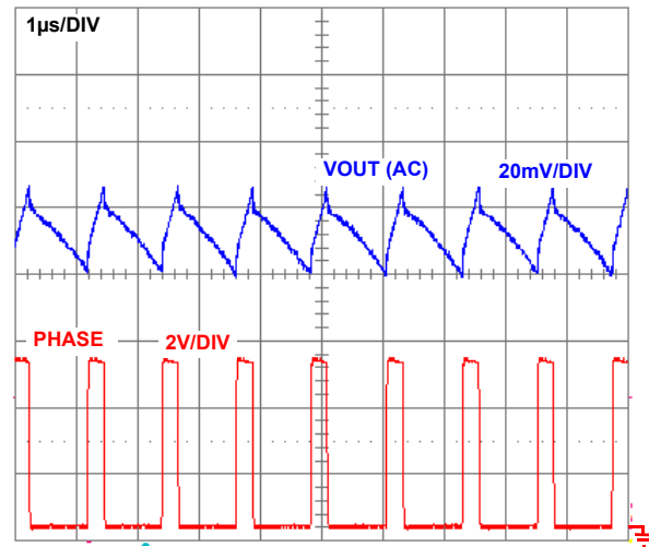
FIGURE 10. CCM STEADY-STATE
