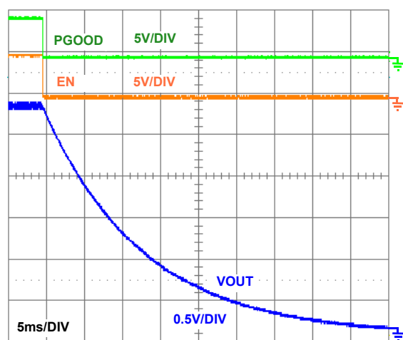
FIGURE 19. NORMAL SHUT-DOWN
