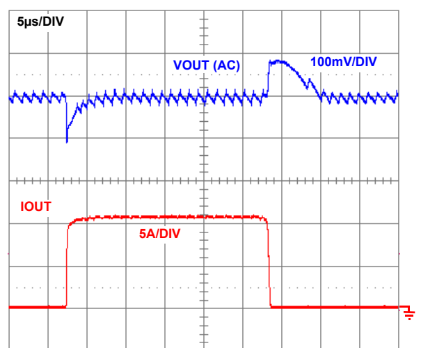
FIGURE 14. 10A LOAD TRANSIENT 50A/μs
