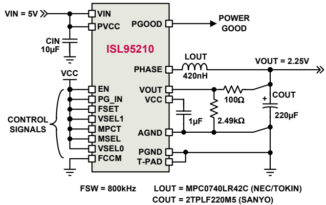
FIGURE 34. ISL95210 TYPICAL APPLICATION WITH VOUT = 2.5V
