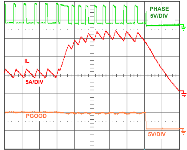
FIGURE 22. OVERCURRENT SHUTDOWN
