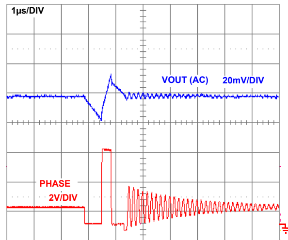
FIGURE 12. AUDIO MODE STEADY-STATE (ZOOM)
