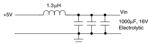
Figure 6. Input Filter
