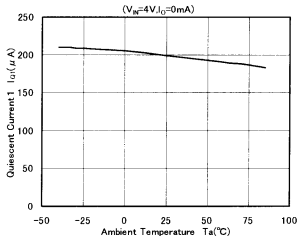
NJM2370 3V Version Quiescent Current 1 vs. Ambient Temperature ( V_{IN}=4\text{V}, I_O=0\text{mA} )
