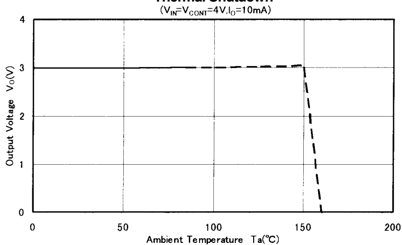
Thermal Shutdown
