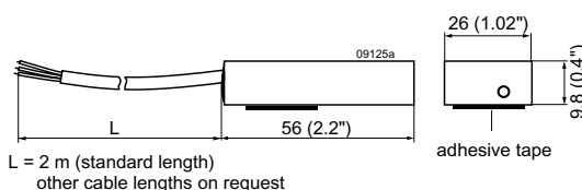
Battery temperature sensor
