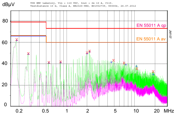
Fig. 16b Typ. conducted emissions (peak/quasipeak and average) at the input according to EN 55011/22, measured at V_i = 110 V and I_{0\text{ nom}} (HR2320-9RG).
