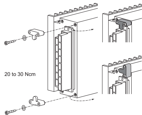
Connector retention brackets CRB HKMS
