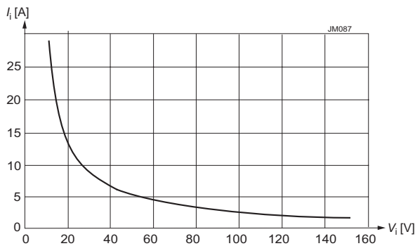
Fig. 2 Typical input current at nominal load versus input voltage
