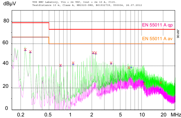
Fig. 16a Typ. conducted emissions (peak/quasipeak and average) at the input according to EN 55011/22, measured at V_i = 24 V and I_{0\text{ nom}} (HR2320-9RG).
