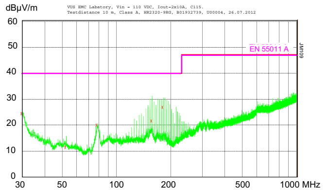
Fig. 17b Typ. radiated emissions accord. to EN 55011/22, antenna 10 m distance, measured at V_i = 110 V and I_{0\text{ nom}} (HR2320-9RG).
