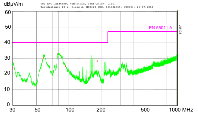
Fig. 17a Typ. radiated emissions accord. to EN 55011/22, antenna 10 m distance, measured at V_i = 24 V and I_{0\text{ nom}} (HR2320-9RG).
