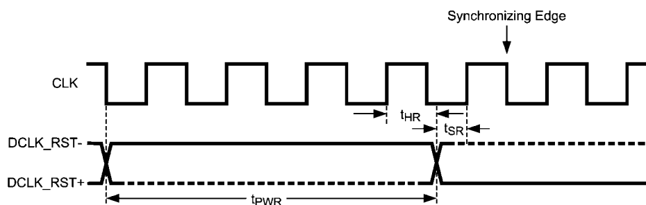
FIGURE 3. Clock Reset Timing
