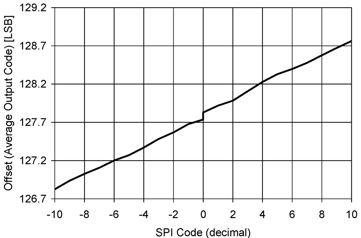
FIGURE 16. Extended Mode Offset Behavior
