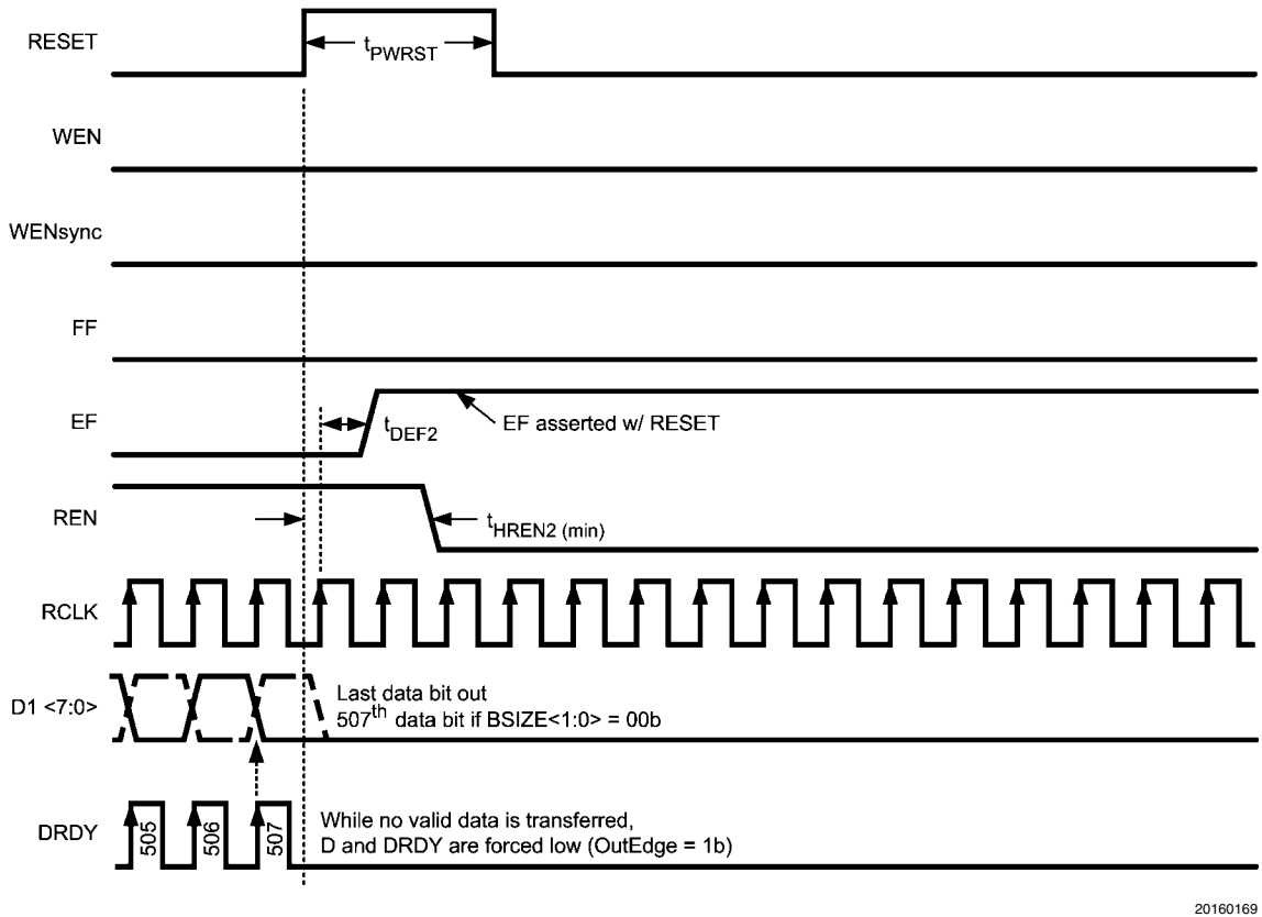
FIGURE 12. Capture Buffer RESET on READ Phase (OutEdge = 1b)(Note 14)
