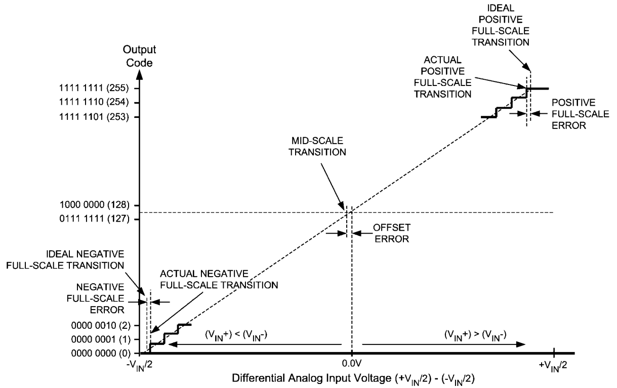
FIGURE 1. Input / Output Transfer Characteristic
