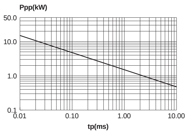
Fig. 3: Peak pulse power versus exponential pulse duration ( T_{j \text{ initial}}=25^{\circ}\text{C} ).
