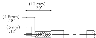
RECOMMENDED STRIP LENGTHS FOR MODEL 7035
