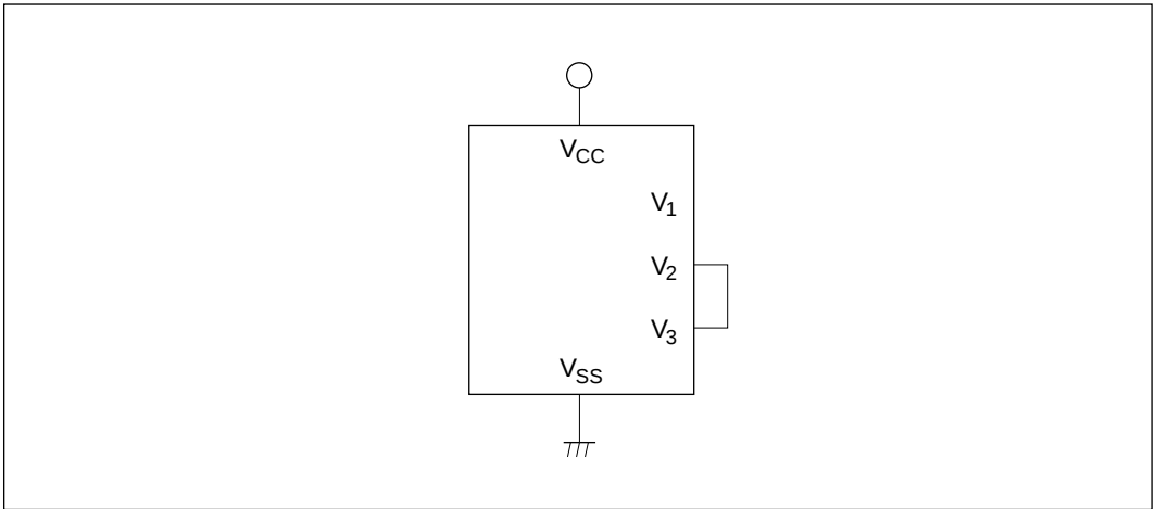
Figure 12-2 LCD Driver Power Supply Processing at 1/2 Duty
