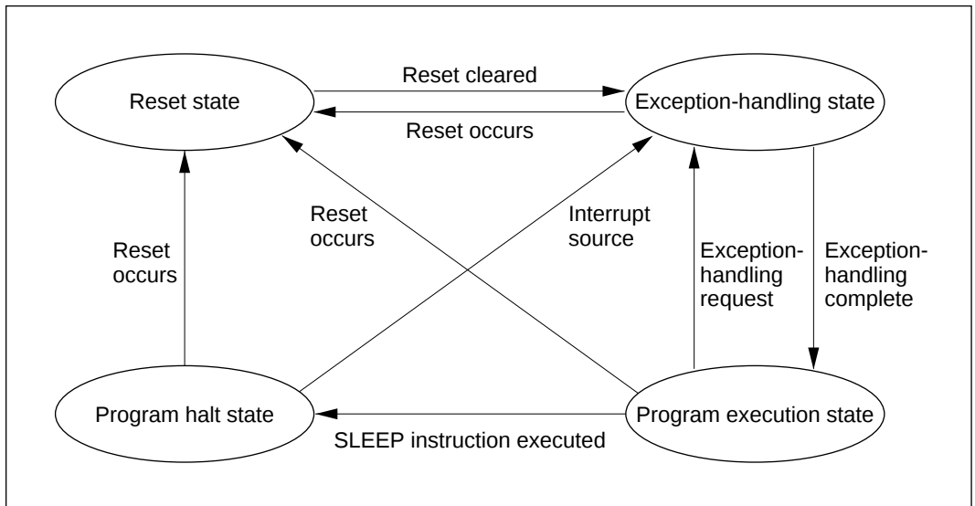
Figure 2-15 State Transitions
