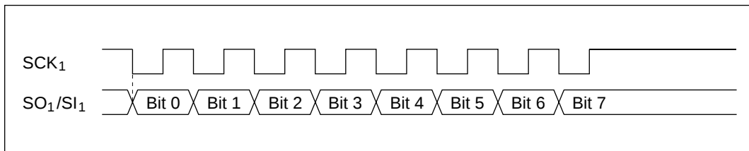
Figure 10-2-2 Transfer Format
