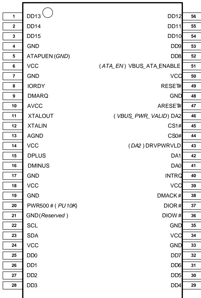
Figure 2. 56-Pin SSOP Pinout (CY7C68300C/CY7C68301C only)
