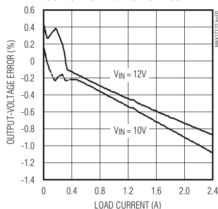
STEP-DOWN REGULATOR NORMALIZED OUTPUT VOLTAGE vs. LOAD CURRENT
