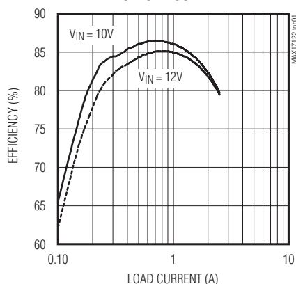
STEP-DOWN REGULATOR EFFICIENCY vs. LOAD CURRENT
