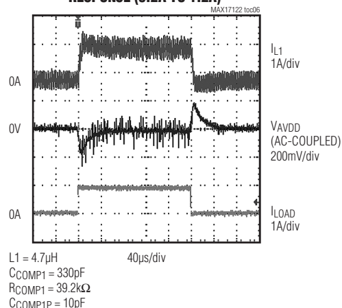
STEP-UP REGULATOR LOAD-TRANSIENT RESPONSE (0.2A TO 1.2A)
