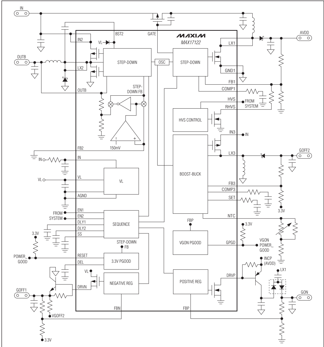
Figure 2. Functional Diagram
