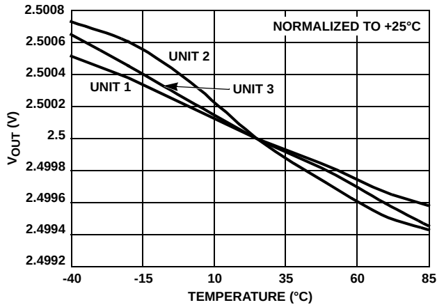
FIGURE 3. V_{OUT} vs TEMP - 3 UNITS
