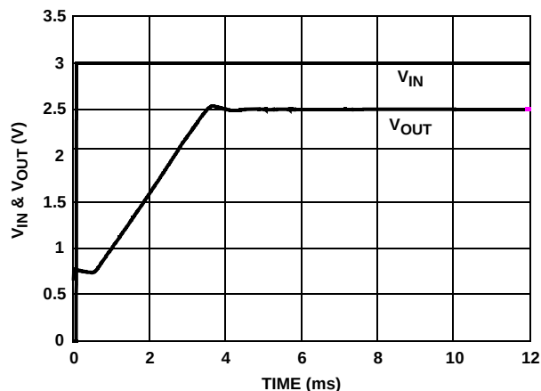
FIGURE 12. TURN-ON TIME @ T_A = 25^\circ C
