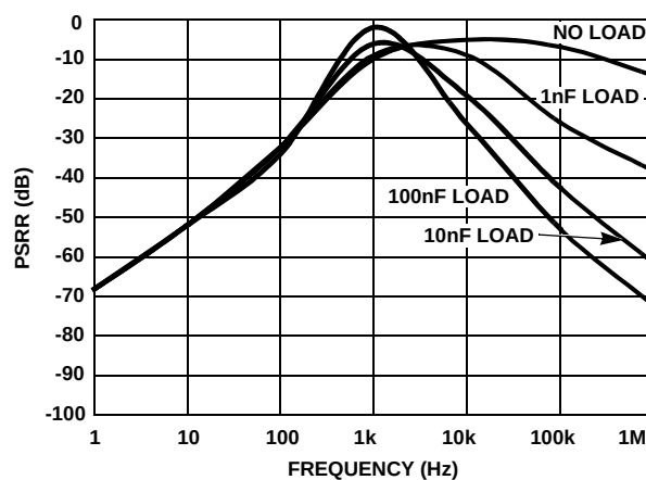
FIGURE 8. PSRR vs f vs C_L
