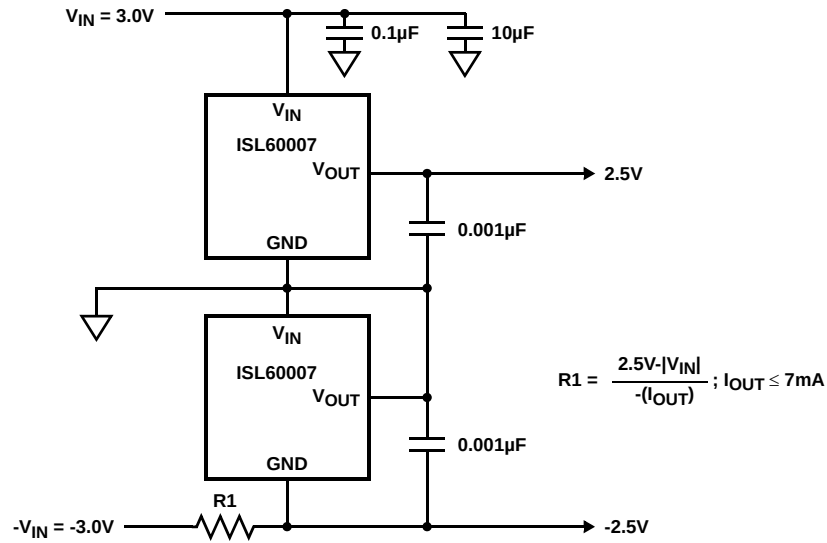
FIGURE 20. \pm 2.5\text{V} DUAL OUTPUT, HIGH ACCURACY REFERENCE
