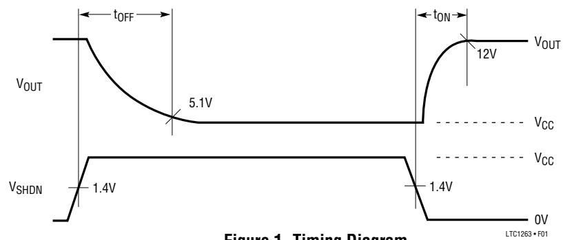
Figure 1. Timing Diagram
