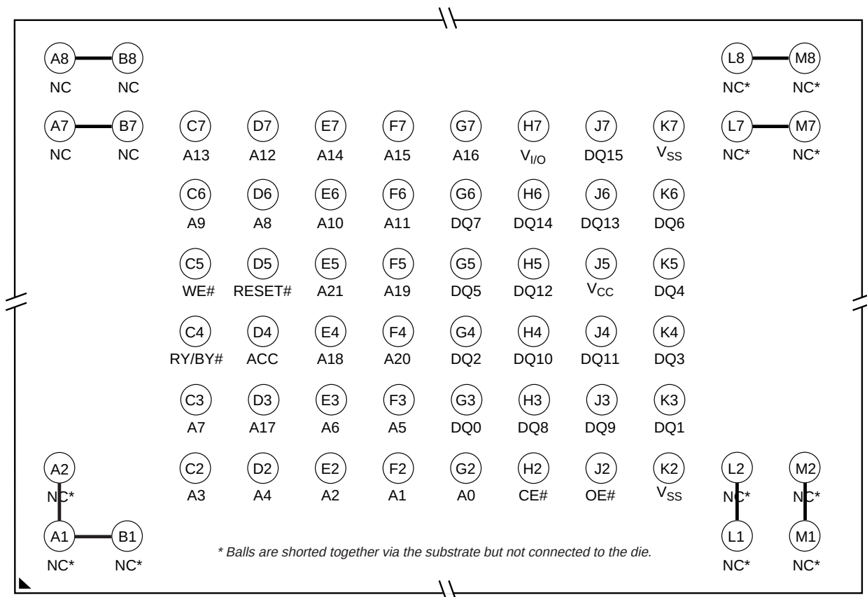
63-Ball FBGA Top View, Balls Facing Down (Am29LV640 only)
