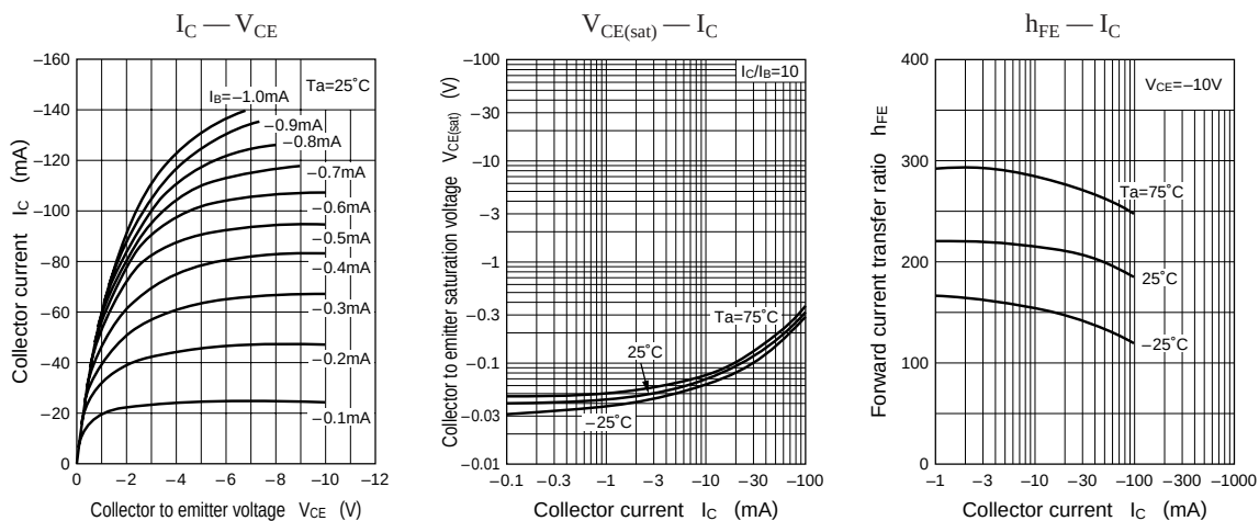
Characteristics charts of UN9116
