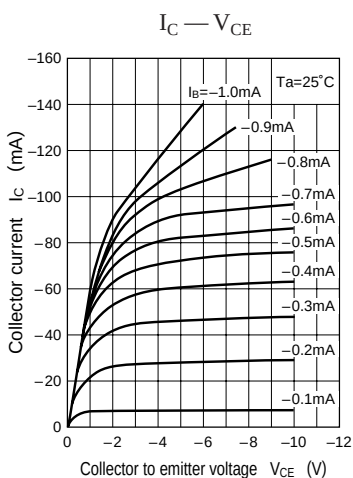
Characteristics charts of UN9111
