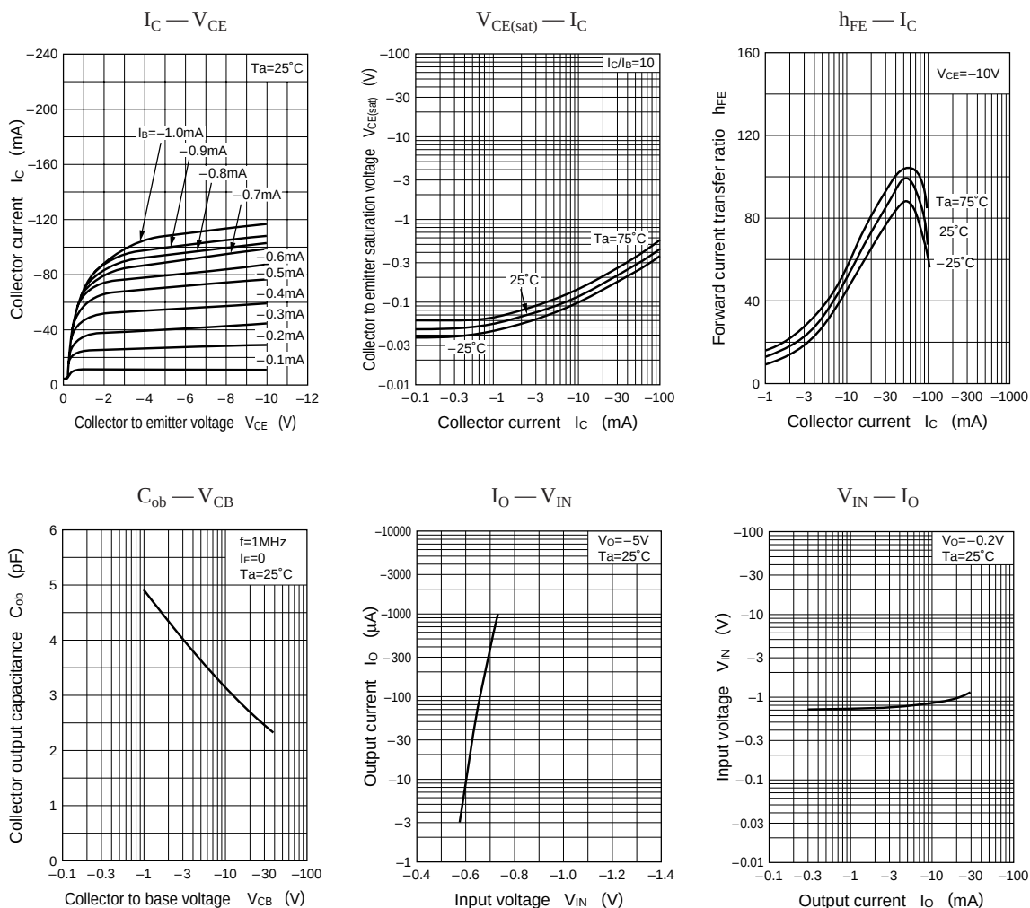
Characteristics charts of UN9119
