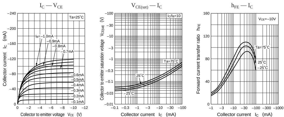
Characteristics charts of UN9119
