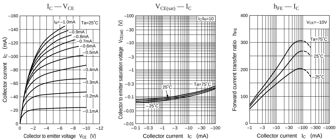
Characteristics charts of UN9113
