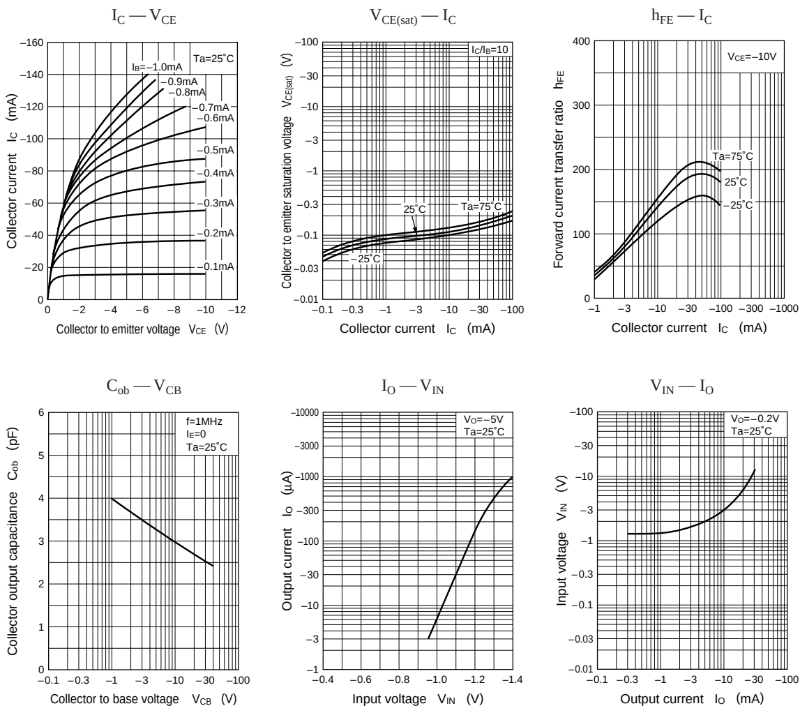
Characteristics charts of UN9113
