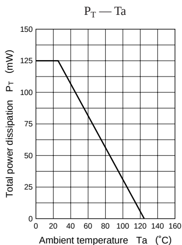
Characteristics charts of UN9111
