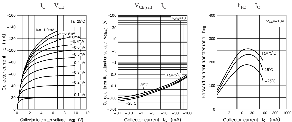
Characteristics charts of UN9114
