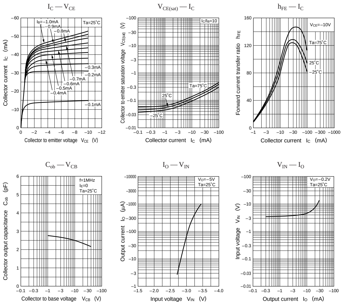
Characteristics charts of UN911E
