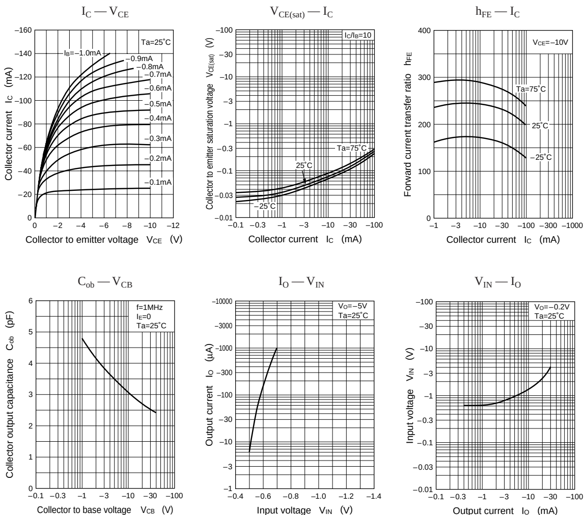
Characteristics charts of UN9116
