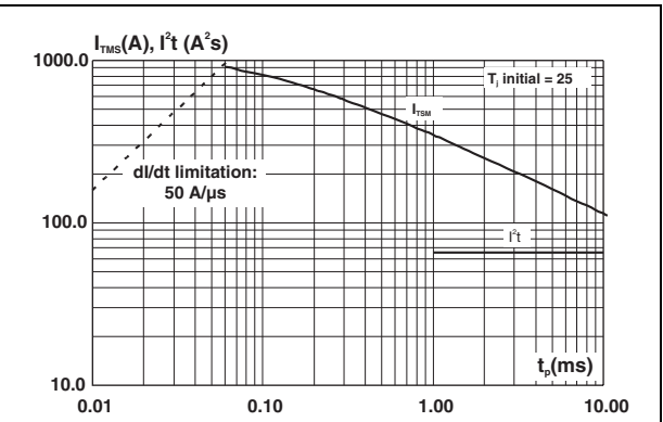
Figure 8. Non-repetitive surge peak on-state current for a sinusoidal pulse, and corresponding values of I^2t
