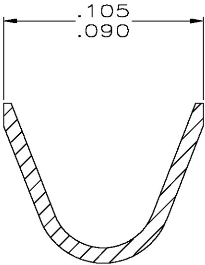
SECTION B-B INSULATION RANGE .025-.060 SCALE 20:1
