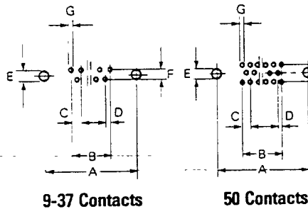
90° Version
