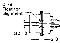
Float Mount
