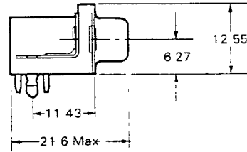
90° PCB mount 15, 26, 44 & 62 contacts
