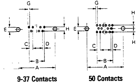
Straight Version
