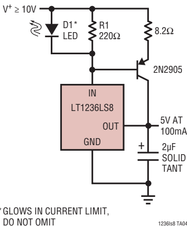
Boosted Output Current with Current Limit
