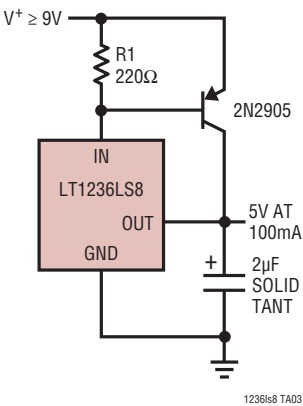
Boosted Output Current with No Current Limit
