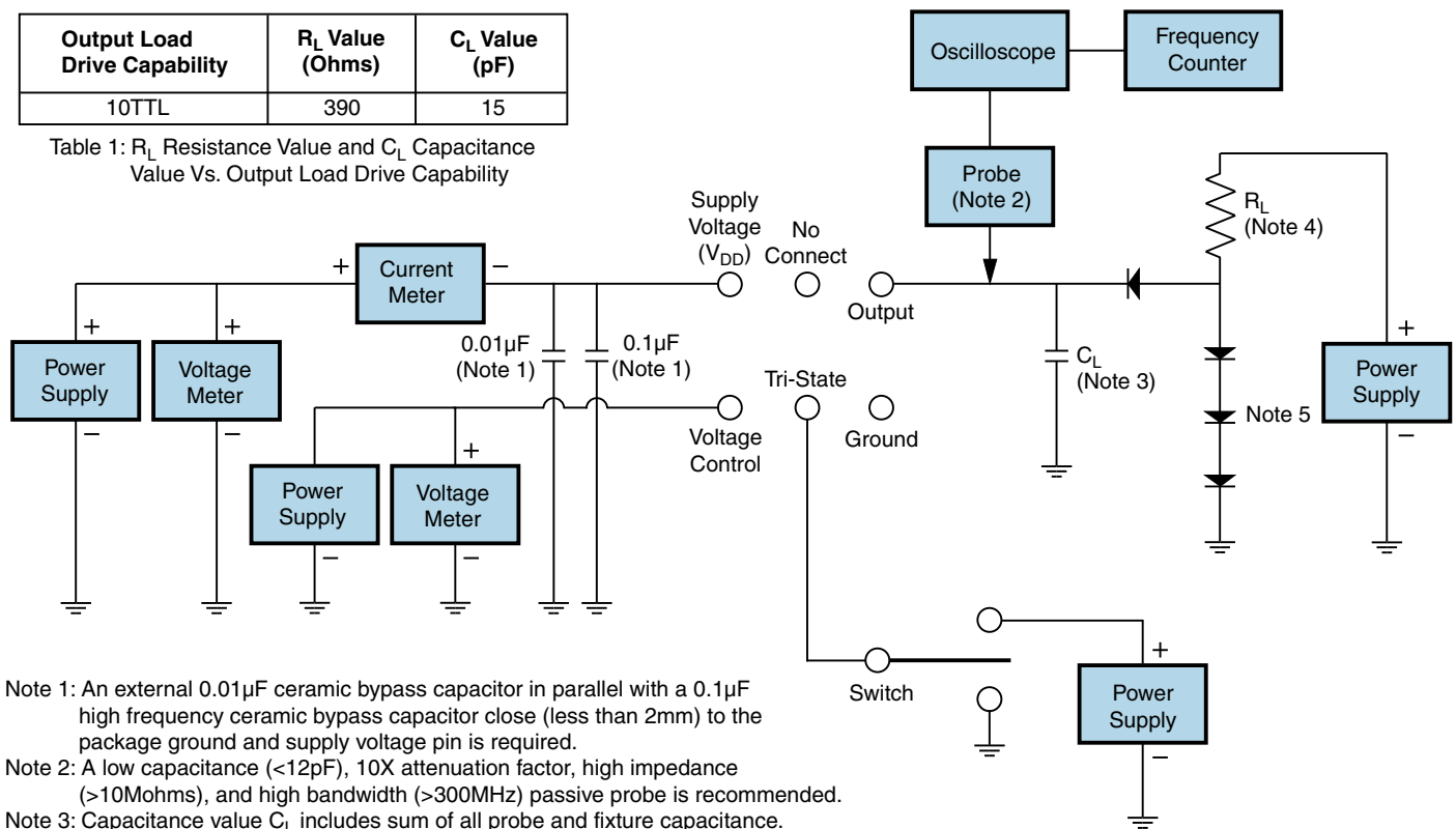
Test Circuit for TTL Output
