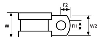
Aluminium P Clips with a Chloroprene insert
