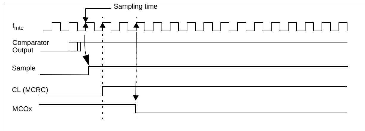
Figure 150. Example 2 : waveforms for overcurrent detection with current feedback filter ON (CFF=001 => 2 consecutive samples are needed to validate the overcurrent event)
