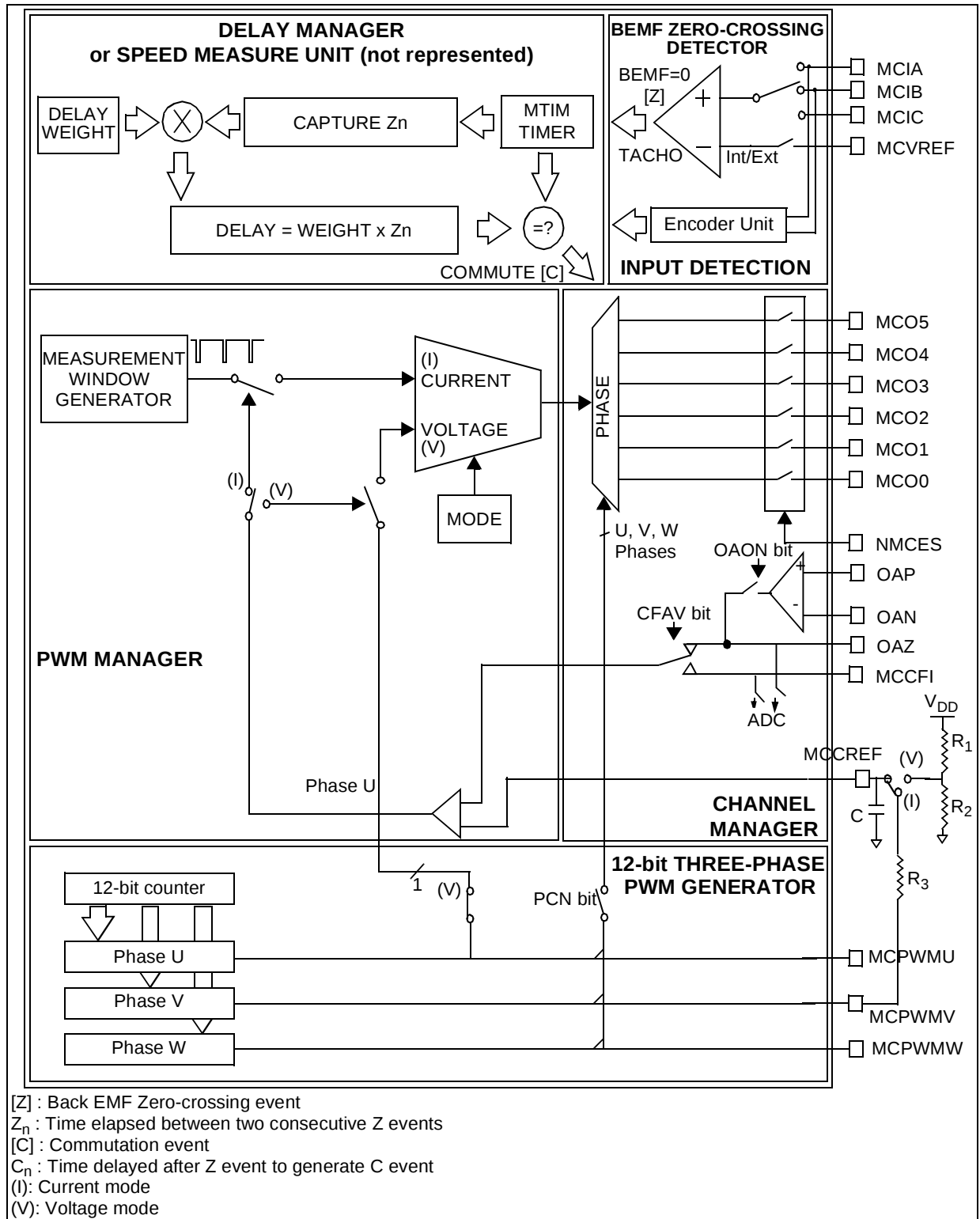
Figure 75. Simplified MTC Block Diagram
