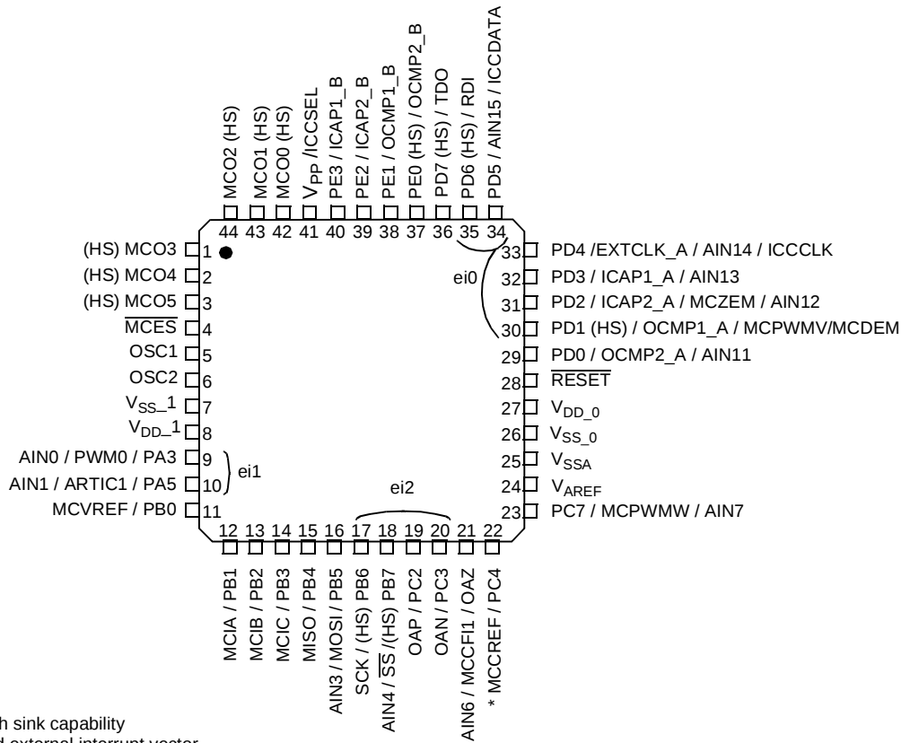
Figure 6. 44-Pin TQFP Package Pinouts
