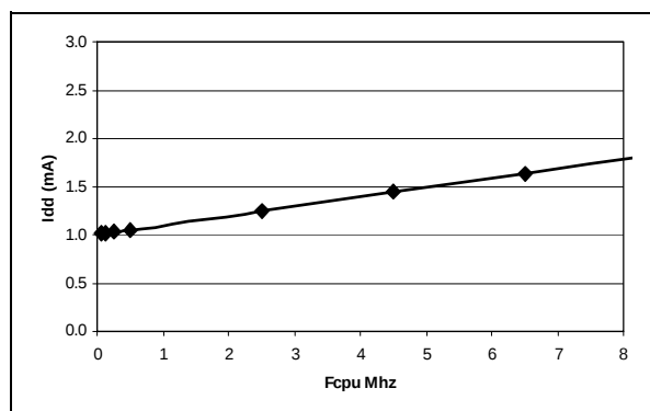
Figure 130. Typical I_{DD} in SLOW vs. f_{CPU}
