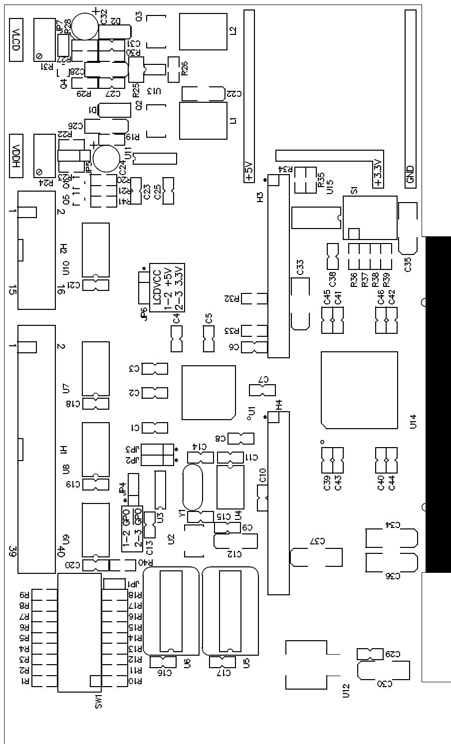
Figure 10-1: S5U13706P00C100 Board Layout
