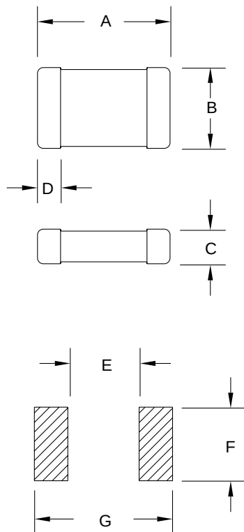
Pad Layout
