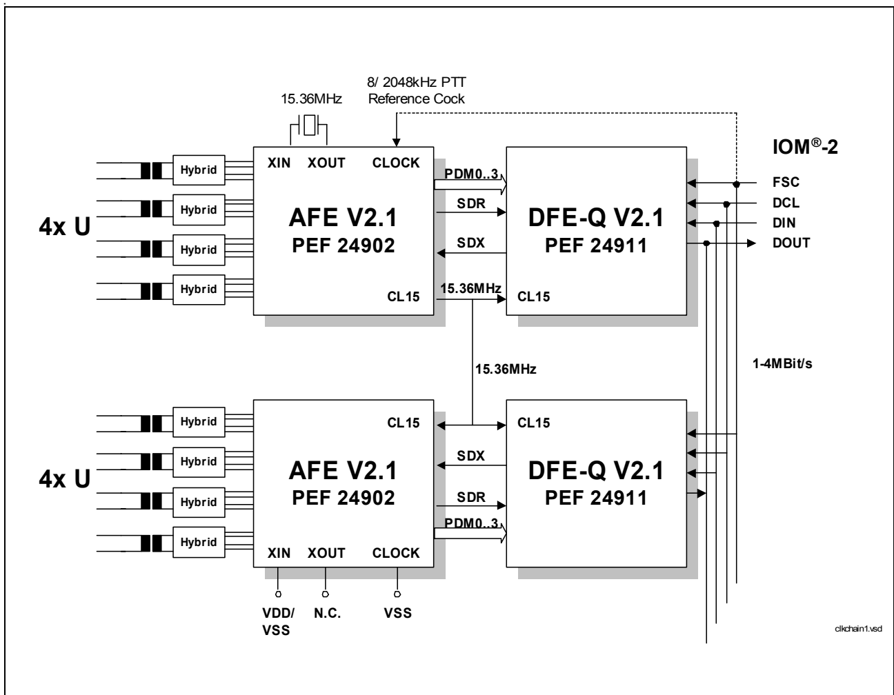
Figure 5 Connecting Two AFE/DFE-Q Chip Sets
