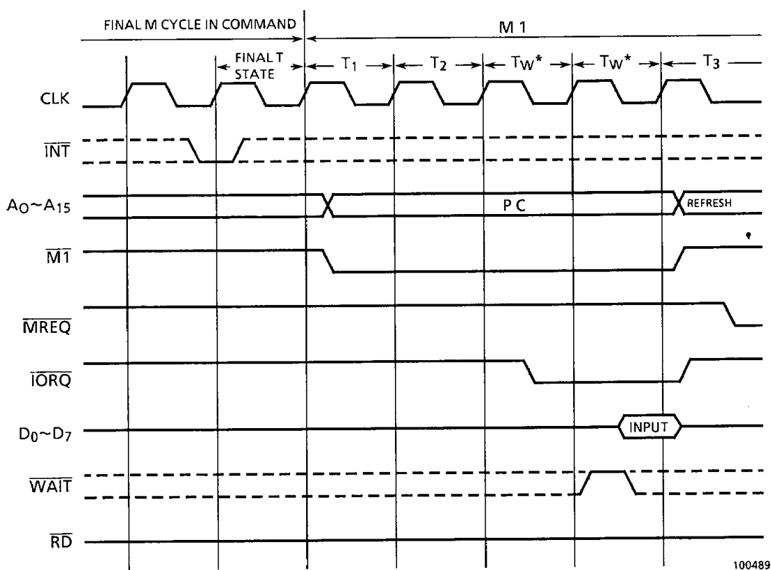
Figure 3.32 Interrupt Acknowledge
