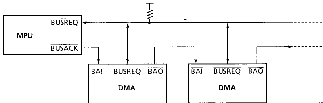
Figure 3.5 BUS REQUEST Daisy Chain
