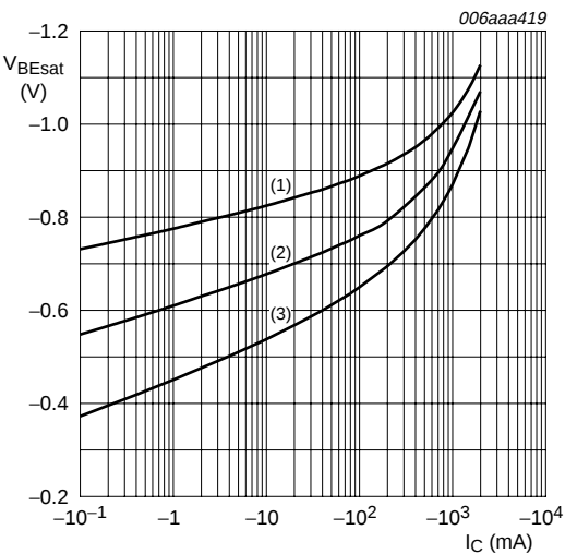
I_C/I_B = 20 (1) T_{amb} = -55^\circ\text{C} (2) T_{amb} = 25^\circ\text{C} (3) T_{amb} = 100^\circ\text{C}
