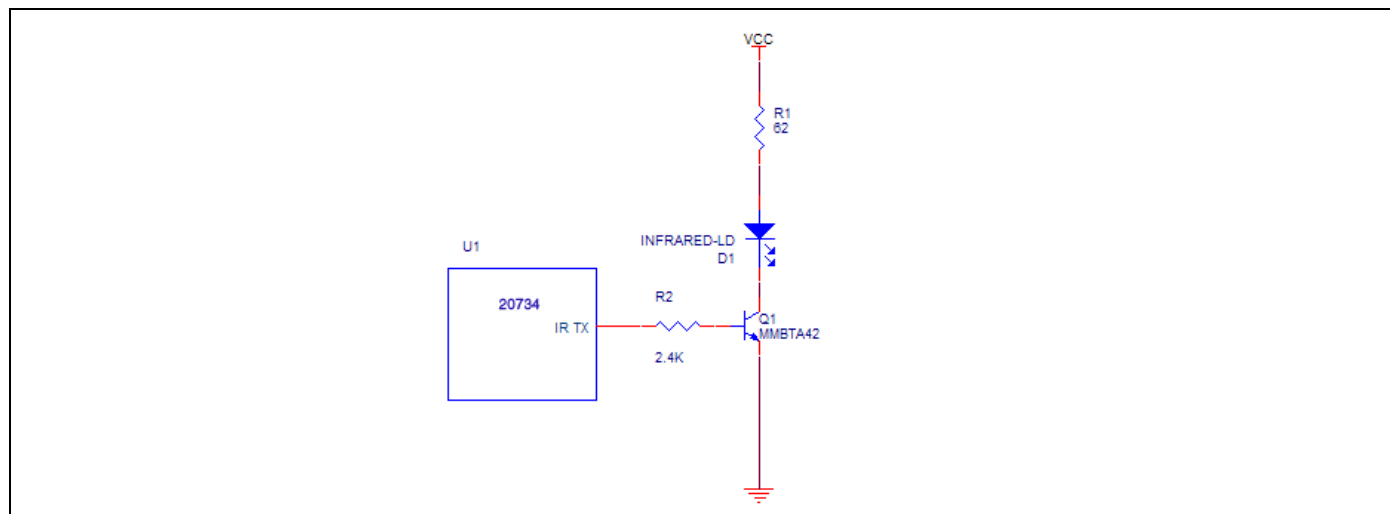
Figure 6. Infrared TX
