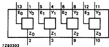
Fig.4 Functional diagram.
