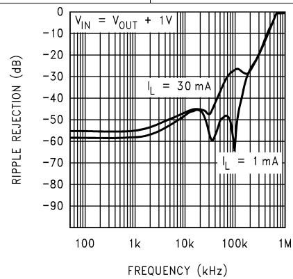
Figure 12. Ripple Rejection
