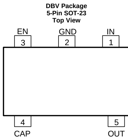
Pin Functions
