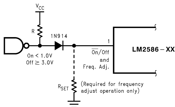
FIGURE 38. Shutdown Operation
