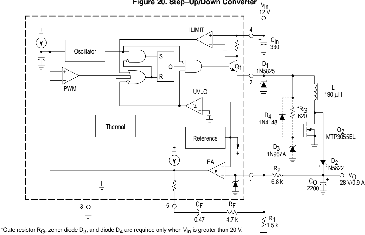
Figure 20. Step-Up/Down Converter
