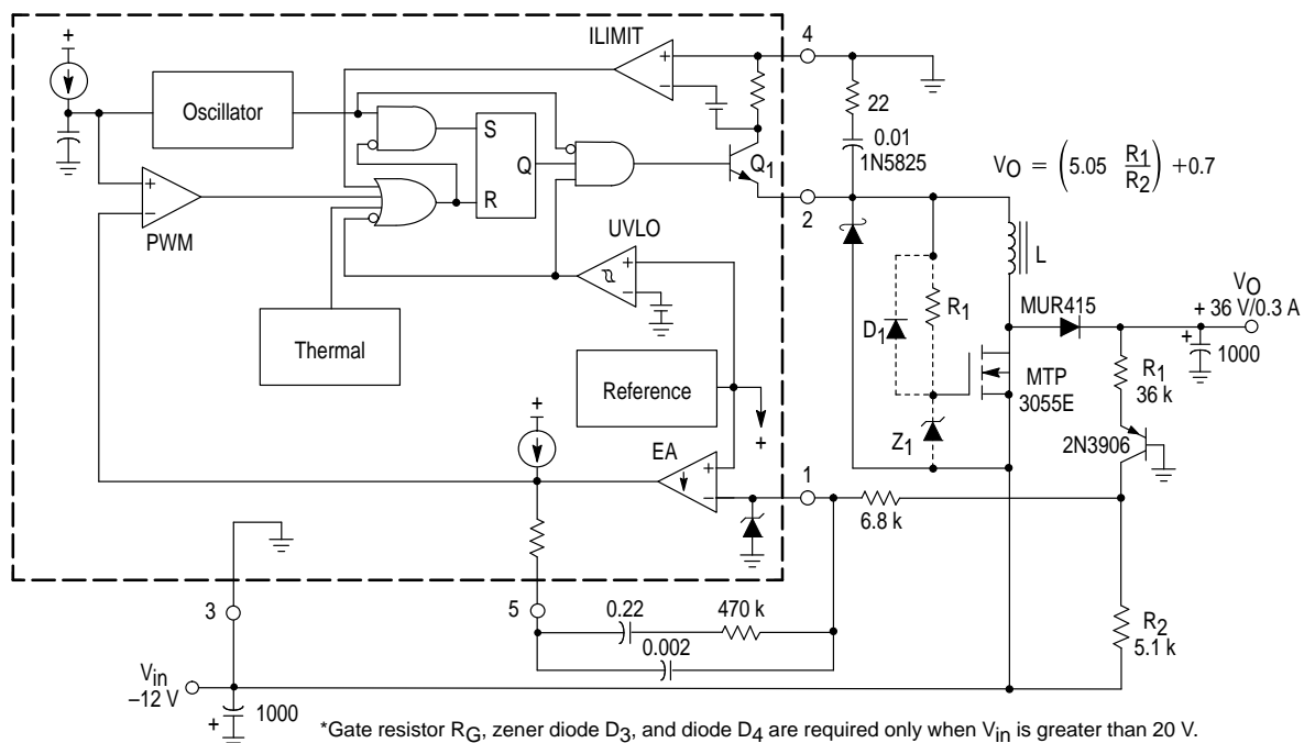
Figure 25. Negative Input/Positive Output Regulator
