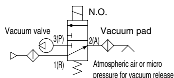
② Valve for vacuum
