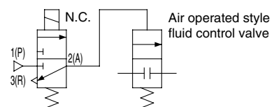
④ Operation for air operated style fluid control valve
