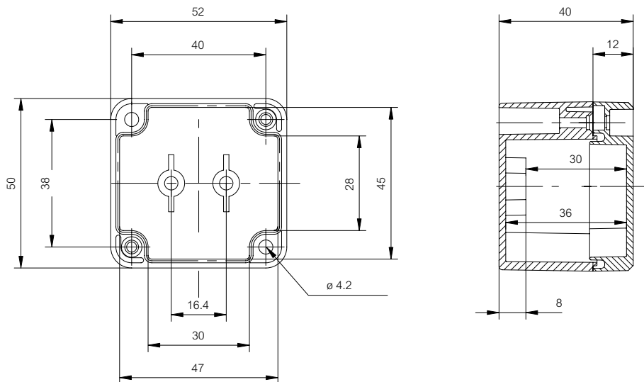
FIBOX EURONORM II 050504
