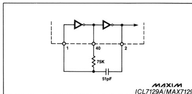
Figure 5B. RC Oscillator Circuit
