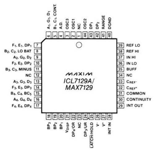
44 Lead Plastic Chip Carrier (Quad Pak)
