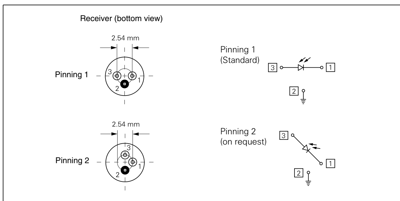
Figure 2 Receiver
