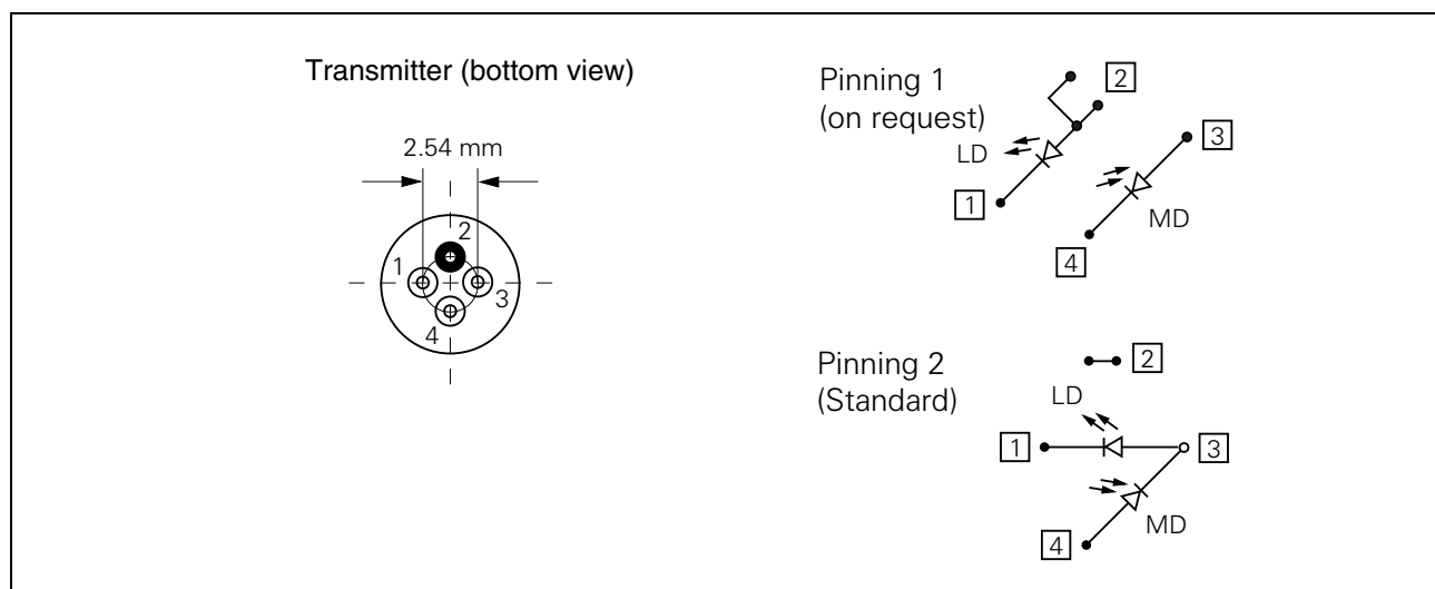
Figure 1 Transmitter
