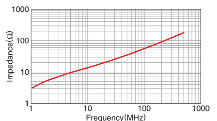
HF70SH42X0.9X12
