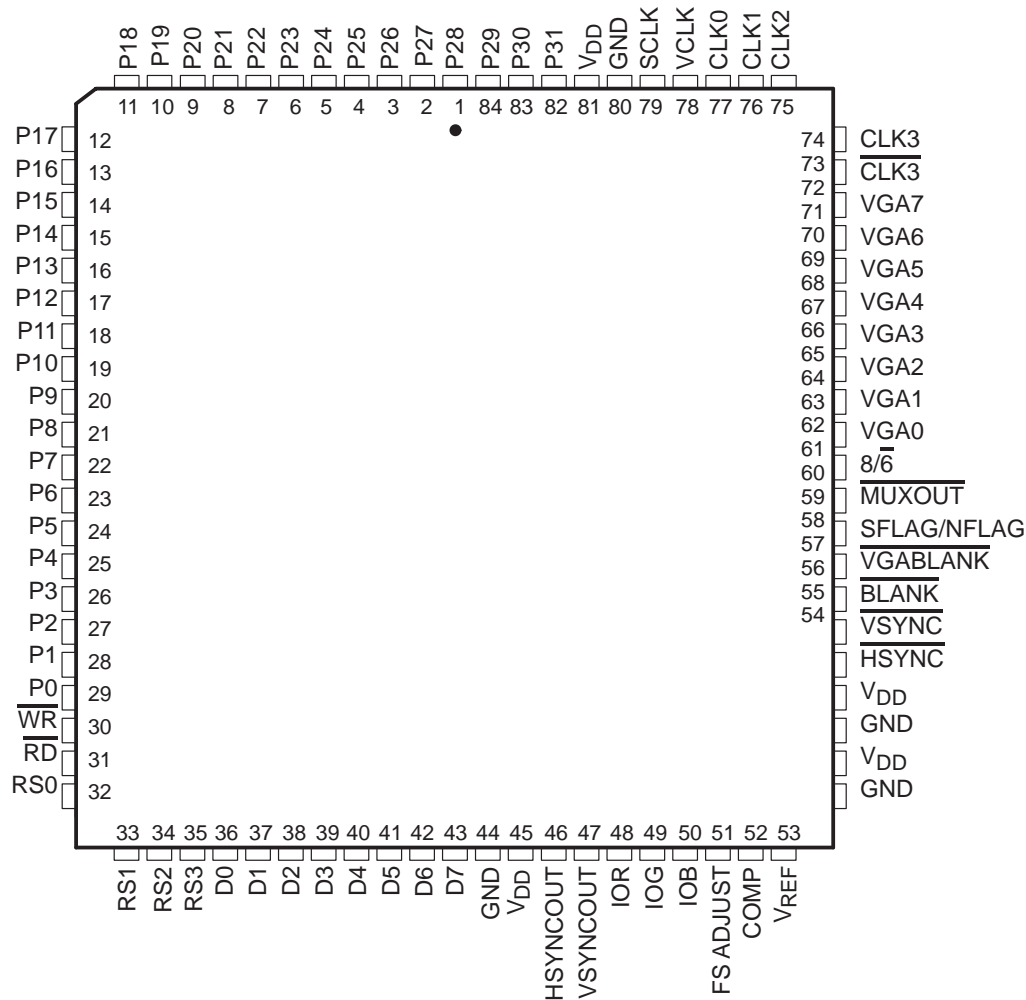
Figure 1–2. Terminal Assignments
