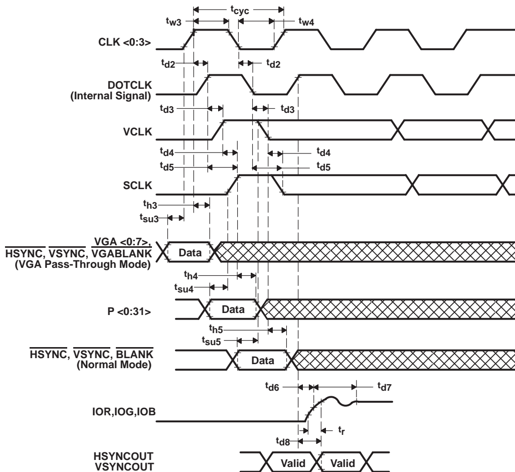
Figure 3–2. Video Input/Output
