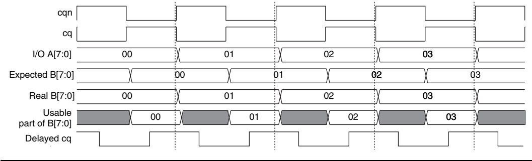
Figure 3–6. Timing Diagram of the IOE
