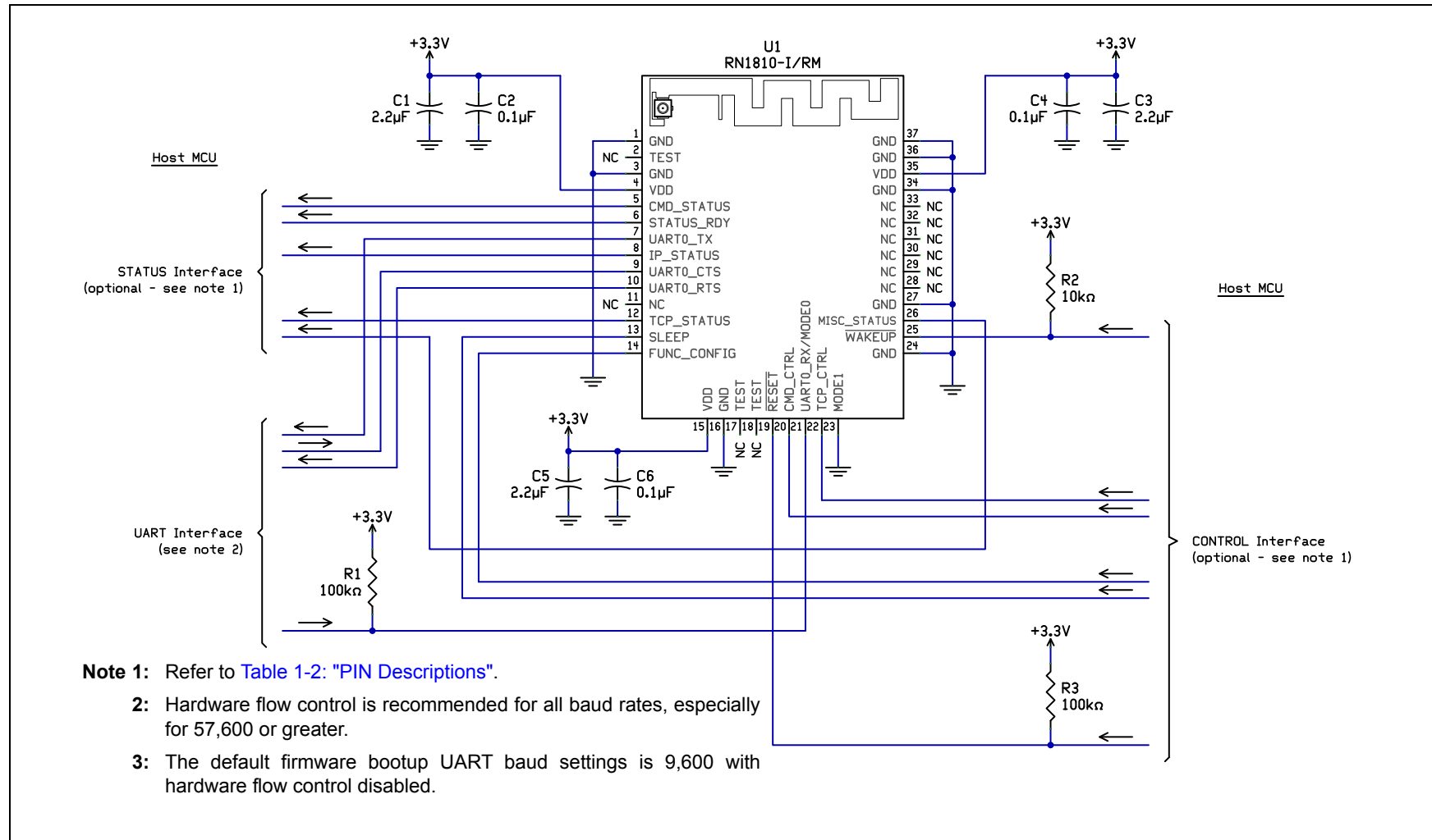
FIGURE 3-1: APPLICATION SCHEMATIC
