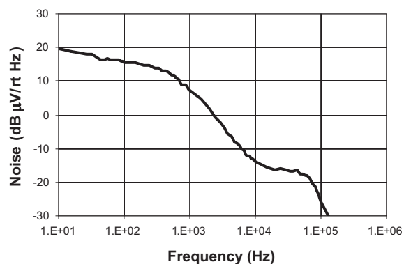
Noise Spectrum
