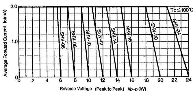
Io - Vp-p Characteristics
