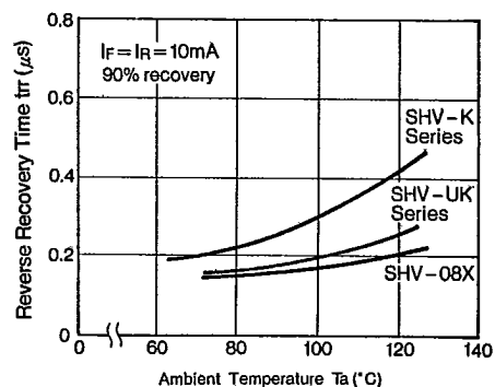
trr - ta Characteristics
