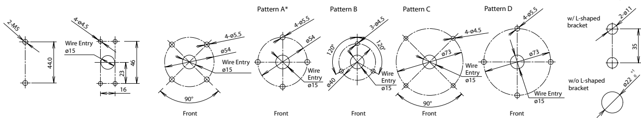
Frame Mount
