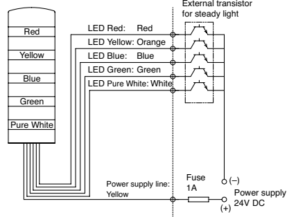
NPN Transistors
