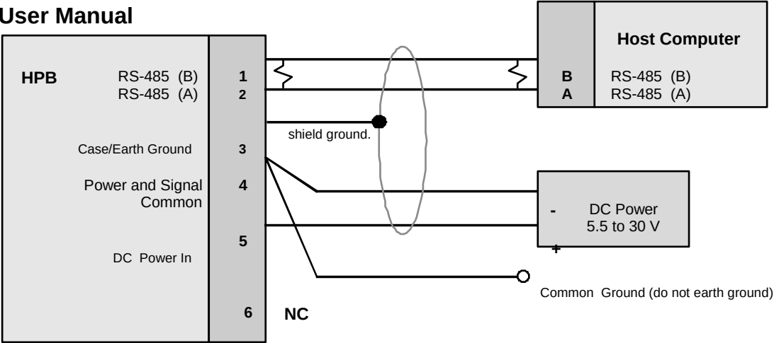
Make all common connections at this end of the cable. Figure 6.3—Connection for RS-485 Operation
