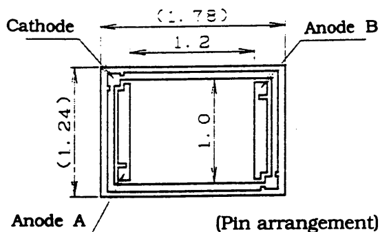
[ Chip drawing (20/1) ]
