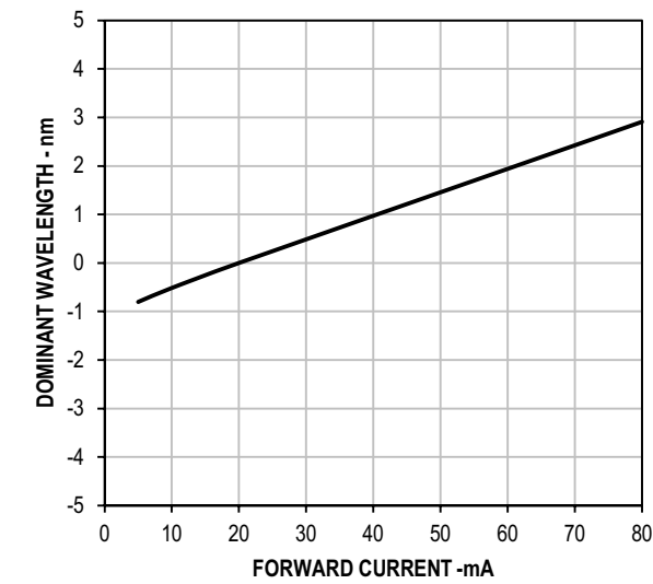
Figure 6: Wavelength vs. Forward Current
